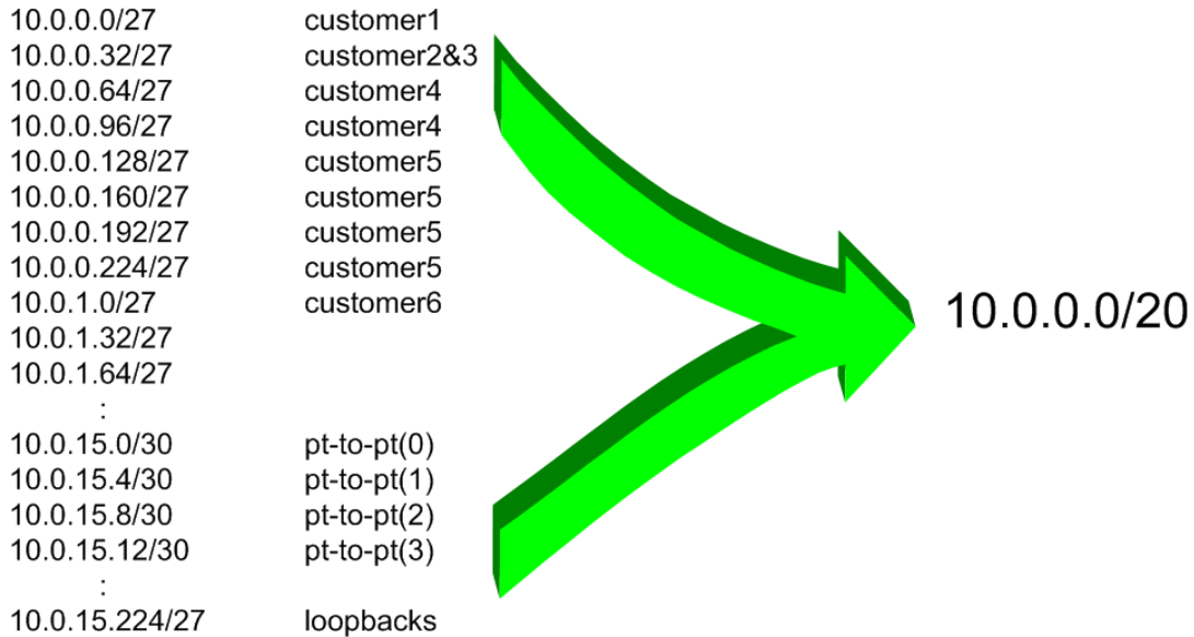
Figure 3 – Extract from an ISP addressing plan
